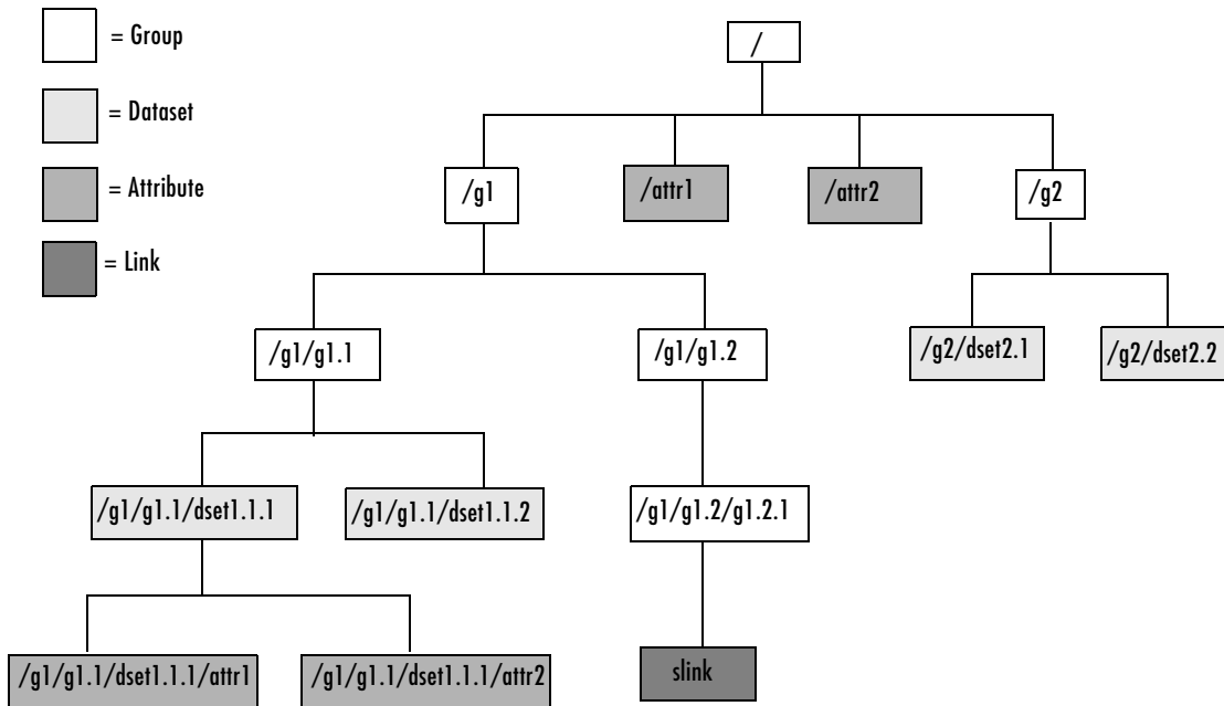
Figure 18-1: Hierarchical Structure of example.h5 HDF5 File
